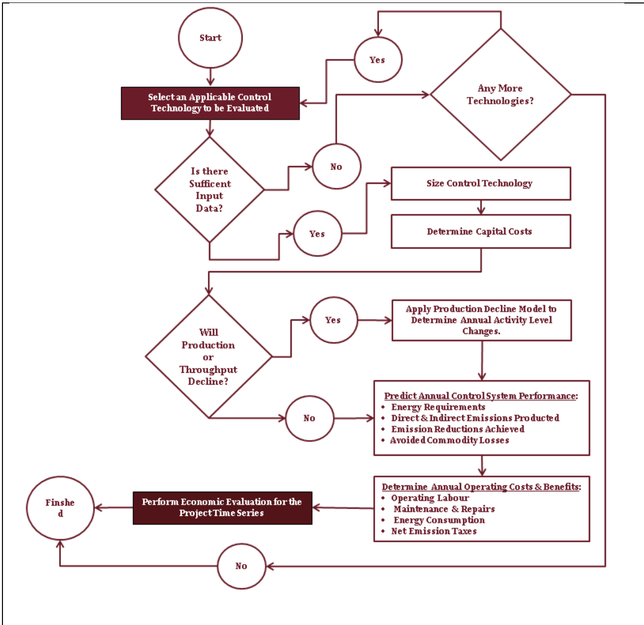
Figure 6: Work flow diagram depicting the control technology selection, sizing and evaluation process.
