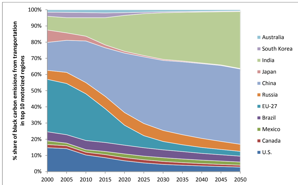
Figure 1-3: Global Black Carbon Emissions from Transportation by Region among Top 10 Motorized Regions, 2000-2050. Source: Data from Facanha et al. (2012).
