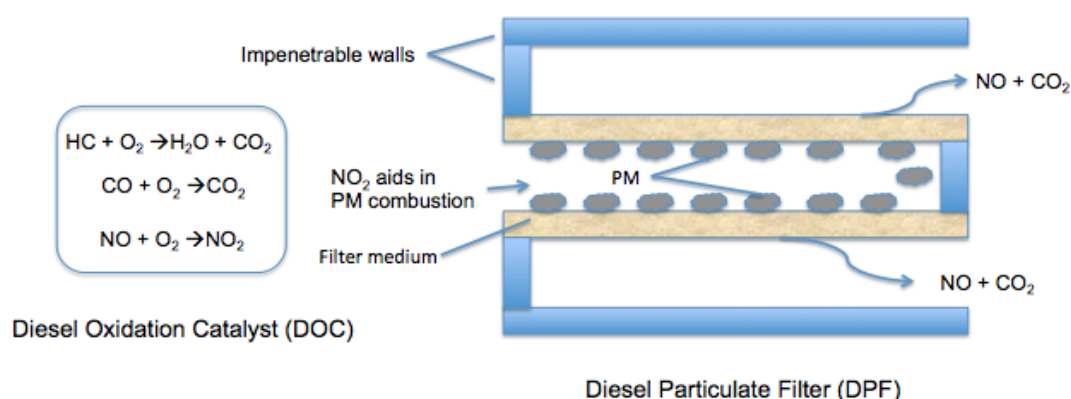
Figure 3-1: Diesel Particulate Filter Operation.
