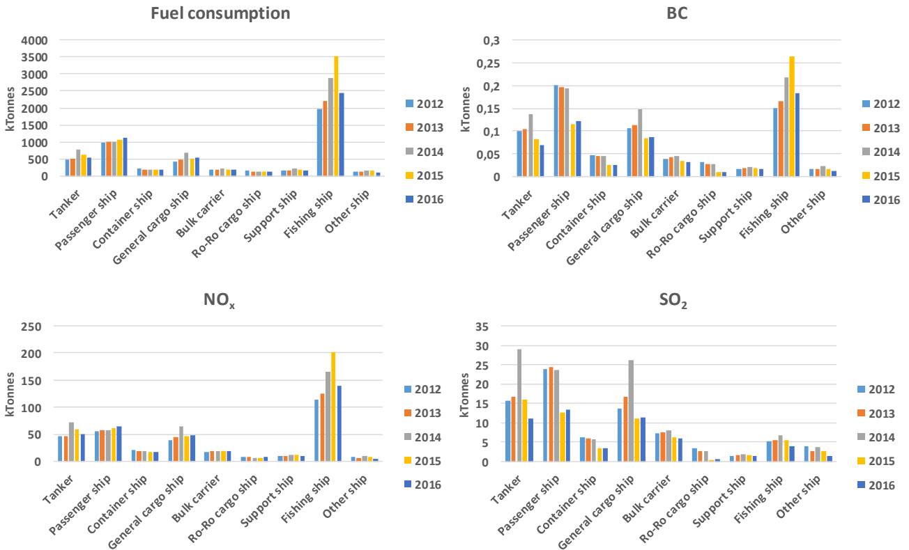
Figure 7.2 Fuel consumption (by mass), \text{NO}_x , \text{SO}_2 and BC emissions per ship type in 2012-2016.
