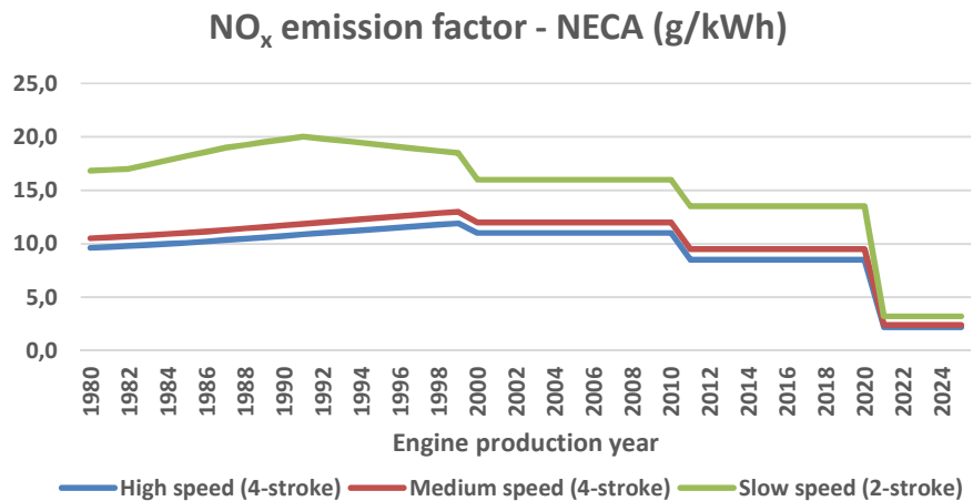
Figure 5.2 NO x emission factors for marine engines per engine production year (g/kWh).
