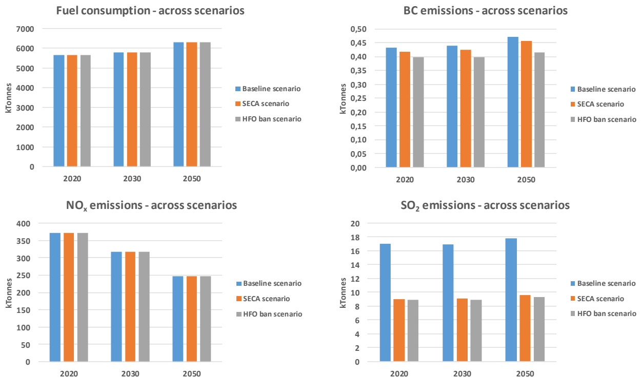
Figure 7.10 Total fuel consumption (by mass), NO x , SO 2 and BC emissions calculated in the Baseline, SECA and HFO ban BAU scenarios.
