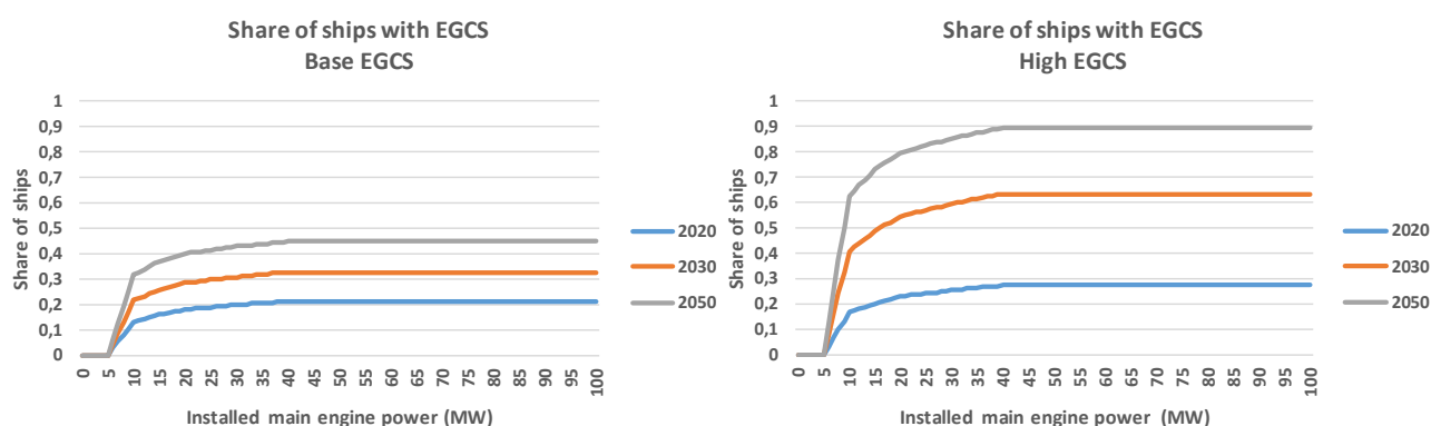
Figure 4.1 Share of ships with EGCS as a function of the installed ship main engine power.
