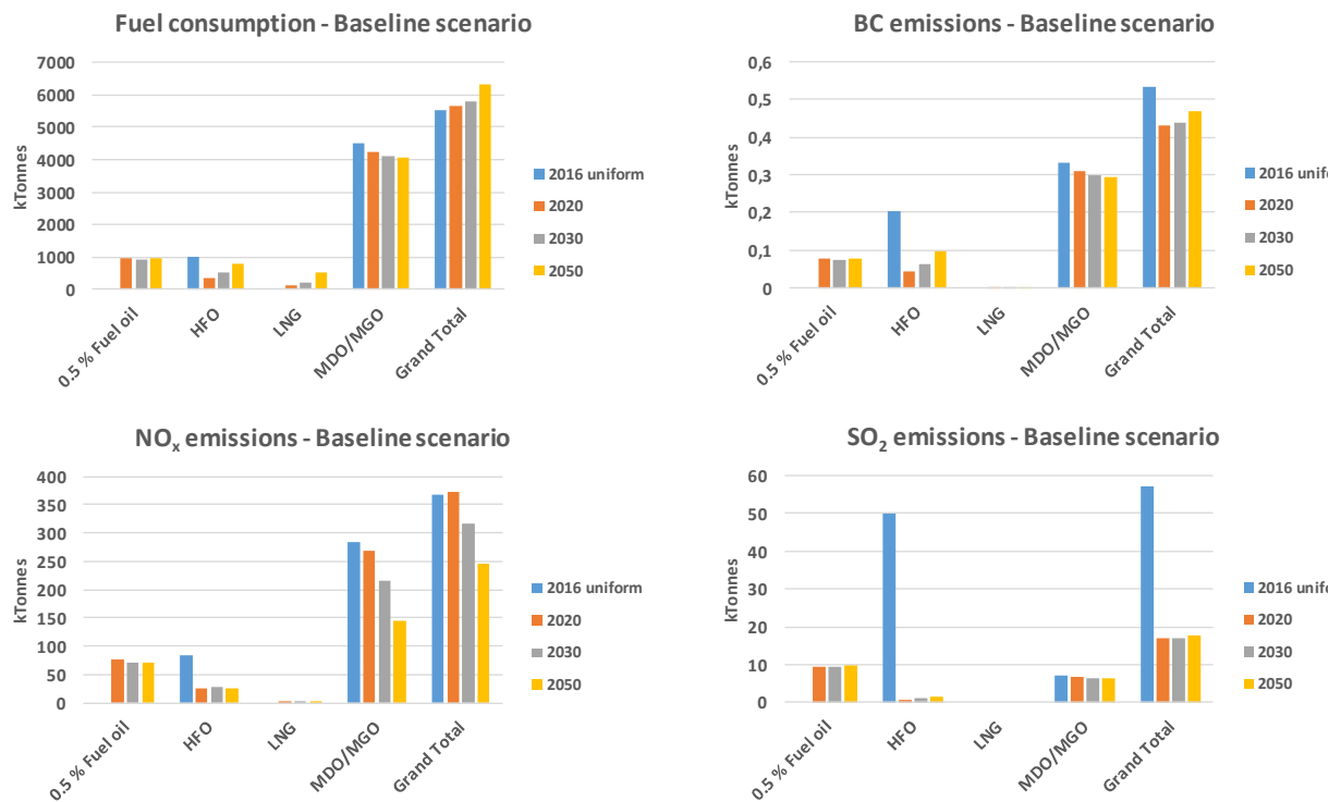
Figure ES 3 Total fuel consumption (by mass), NO x , SO 2 and BC emissions calculated for 2016 (uniform gridded) and 2020, 2030 and 2050 in the Baseline BAU scenario.
