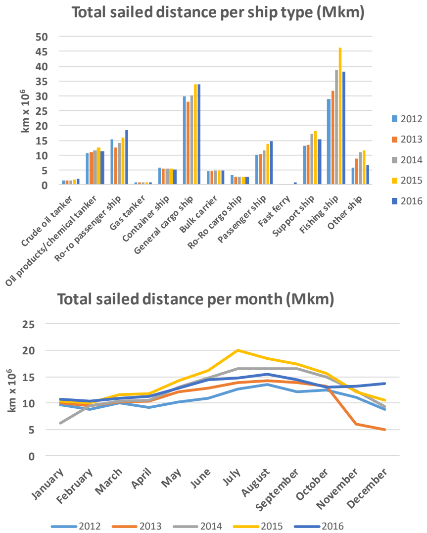
Figure 2.2 Distance sailed per ship type in 2012-2016 (upper figure) and total distance sailed per month 2012-2016 (lower figure).
