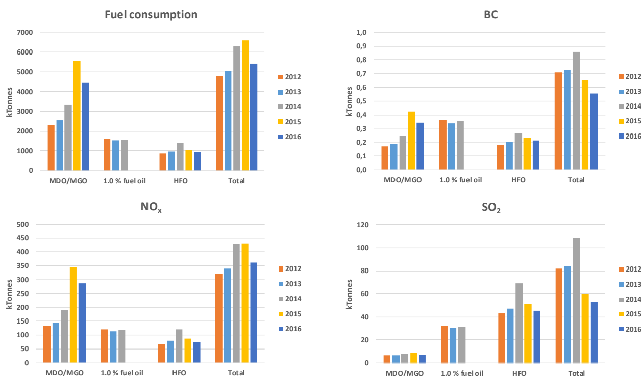
Figure ES 1 Total fuel consumption (by mass), NO x , SO 2 and BC emissions in 2012-2016.
