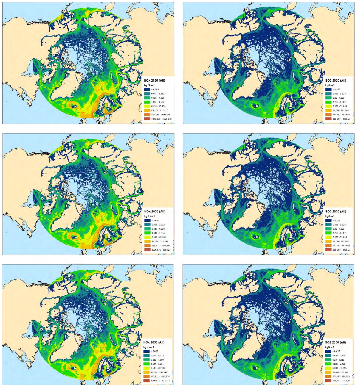
Figure 7.6 Spatial distribution of NO x and SO 2 emissions for all ships in 2020, 2030 and 2050 calculated in the Baseline BAU scenario.
