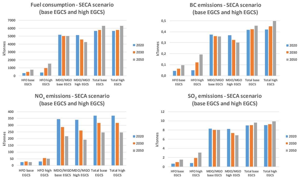
Figure 7.8 Total fuel consumption (by mass), NO x , SO 2 and BC emissions calculated in the baseline and high EGCS model runs.
