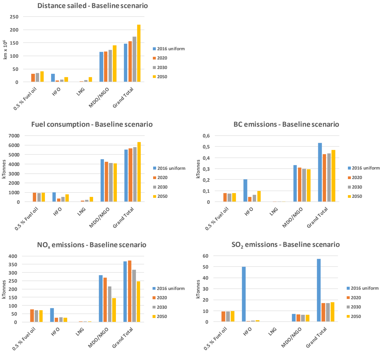
Figure 7.5 Total fuel consumption (by mass), NO x , SO 2 and BC emissions calculated in the Baseline BAU scenario.
