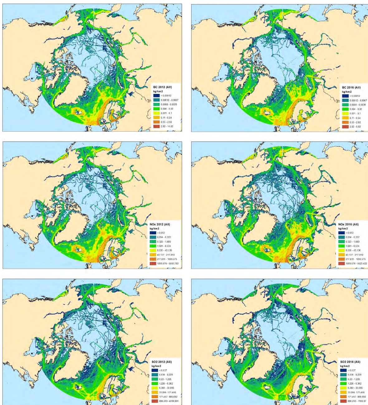
Figure 7.4 Spatial distribution of BC, NO x and SO 2 emissions for all ships in 2012 and 2016.
