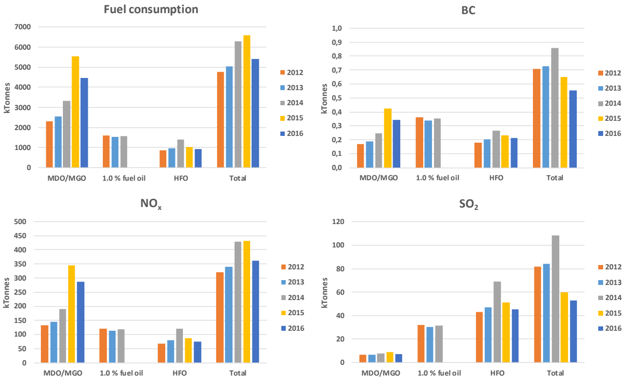
Figure 7.1 Total fuel consumption (by mass), \text{NO}_x , \text{SO}_2 and BC emissions in 2012-2016.
