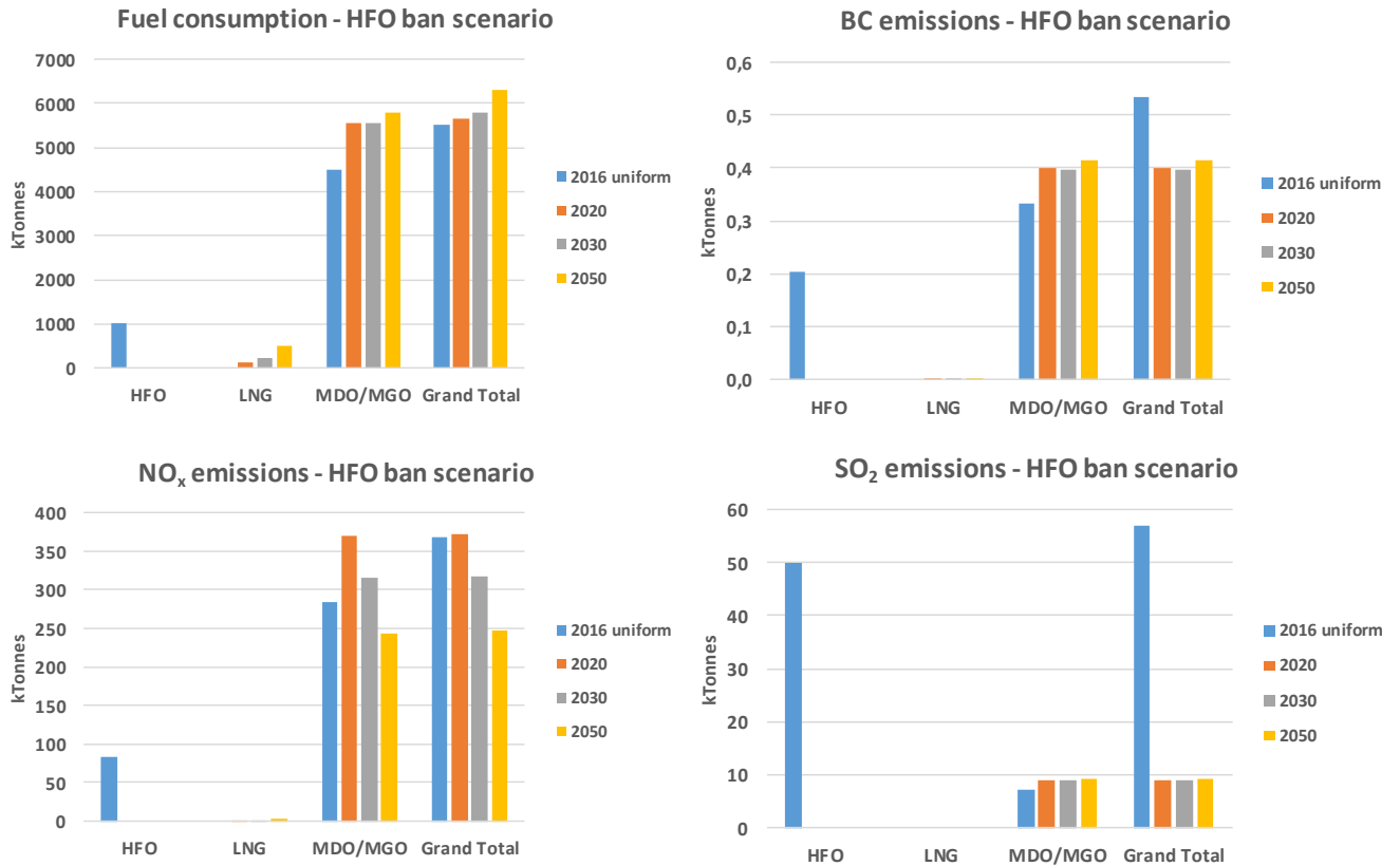
Figure 7.9 Total fuel consumption (by mass), NO x , SO 2 and BC emissions calculated in the HFO ban BAU scenario.
