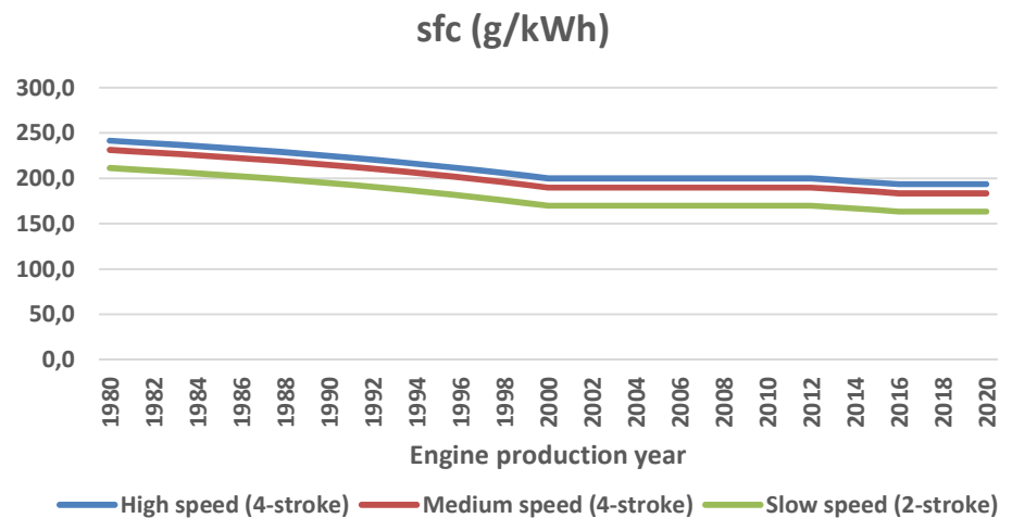
Figure 5.1 Specific fuel consumption for marine engines per engine production year (g/kWh).
