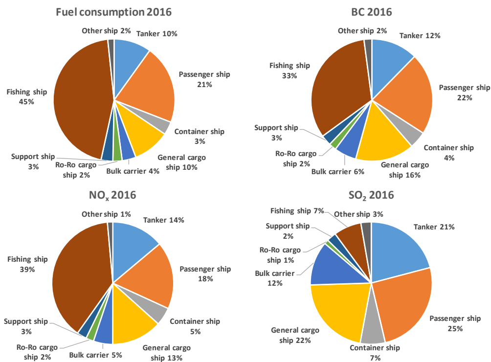
Figure 7.3 Shares of fuel consumption (by mass) and NO x , SO 2 and BC emissions per ship type in 2016.
