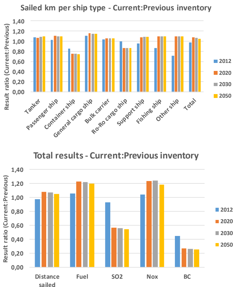
Figure 7.12 Ratios of results for sailed km per ship type (upper figure) and total distance, fuel consumption, SO 2 , NO x and BC emissions (lower figure) between current and previous inventory for the years 2012, 2020, 2030 and 2050.
