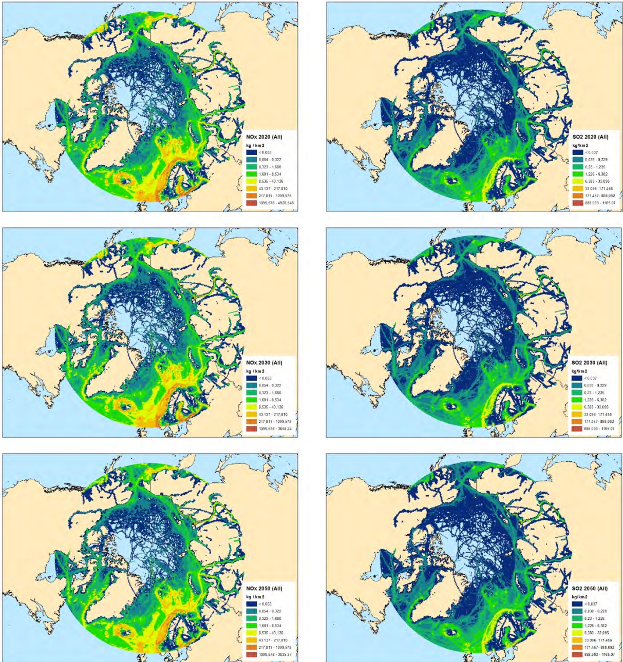
Figure ES 4 Spatial distribution of NO x and SO 2 emissions for all ships in 2020, 2030 and 2050 calculated in the Baseline BAU scenario.
