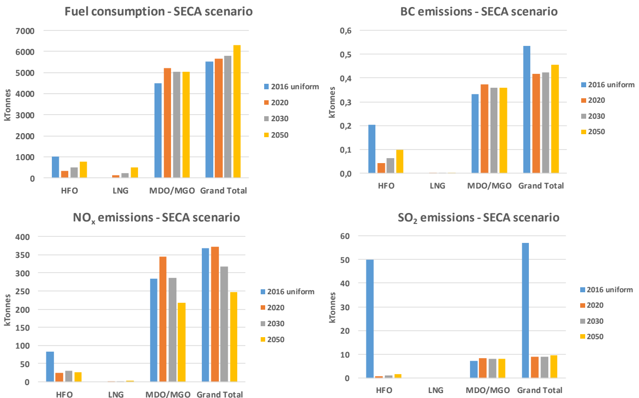
Figure 7.7 Total fuel consumption (by mass), NO x , SO 2 and BC emissions calculated in the SECA BAU scenario.
