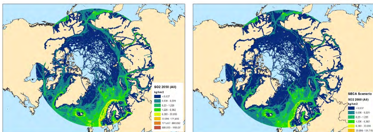
Figure 7.11 Spatial distribution of SO 2 emissions for all ships in 2050 calculated in the Baseline and SECA scenarios.
